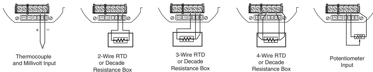
Figure 4. Sensor/input connections
